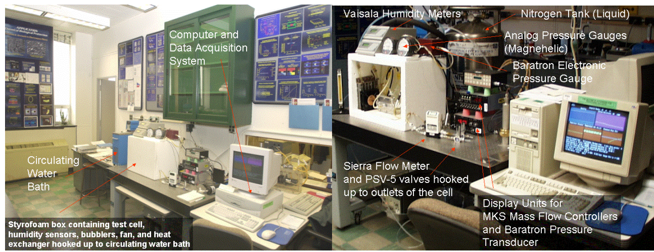
Dynamic Moisture Permeation Cell (DMPC)
