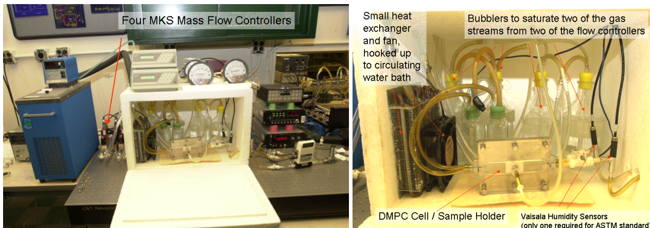
Conditioning Chamber and Sample Holder
